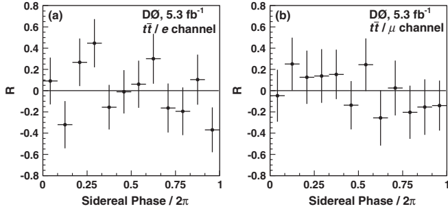
FIG. 1. The dependence of R , as defined in Eq. (6), on the sidereal phase for (a) e + >3 jets t\bar{t} candidates and (b) \mu + >3 jets t\bar{t} candidates.
