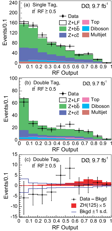
FIG. 1 (color online). Distributions of the global RF discriminant in the t\bar{t} depleted region, assuming M_H = 125 \text{ GeV} , after the fit to the background-only model for the data (points with statistical error bars) and background (histograms) for (a) single-tagged events and (b) double-tagged events. (c) Background-subtracted distribution for (b). The signal distribution is shown with the SM cross section scaled by a factor of 5. The blue lines indicate the uncertainty from the fit.
