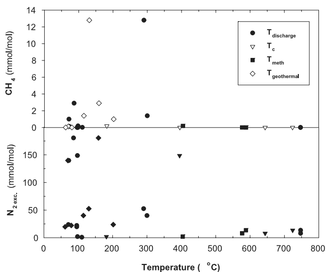
Fig. 3. Discharge and calculated equilibration temperatures vs. CH 4 (upper) and N 2 exc. (lower plot). The general lack of correlations between T and N 2 exc. , T and CH 4 , or N 2 exc. and CH 4 reveals that the nitrogen in Nicaraguan volcanic and geothermal gases is not affected by temperature-dependent crustal contamination. Temperature calculation methods are shown in Table 5.
