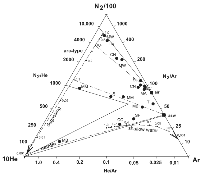
Fig. 4. Triangular plot of N 2 , He, and Ar for the Nicaraguan gases. Air, air-saturated water (asw), mantle wedge gases, and arc-type gases are all marked on the diagram as discussed in the text. Calculated fractionation trends for degassing magma and exsolution from shallow water (see Section 5.1.4 for calculations) are shown as dashed lines with arrows pointing in the direction of progressive fractionation (decreasing F , the fraction of gas remaining in the melt or water), and labelled tick marks show calculated values for F . Dash-dot lines represent examples of mixing trends between air or asw and variably degassed magmatic gas. Symbols after Fig. 2, with MA, Masaya; X, Xiloá; MW, Momotombo geothermal wells; SF, San Francisco Libre; CN, Cerro Negro; and SC, San Cristóbal.
