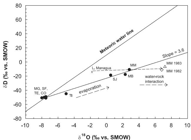
Fig. 2. Plot of \delta D vs. \delta^{18}O showing stable isotopes of Nicaraguan thermal waters (Monte Galan, San Francisco Libre, Telica, Tipitapa, Cosegüina, and San Jacinto) and vapor condensates (Mombacho and Momotombo). Data points form an evaporation trend (thin solid line; slope = 3.6, r^2 = 0.98 ) departing from the meteoric water line (MWL; Craig, 1961). Momotombo may alternately be derived from water–rock interaction by water from Lake Managua (X, dashed line). Also plotted are Momotombo vapor condensate measurements from 1983 (Allard, 1983) to 1982 (Menyailov et al., 1986). Symbols: MG, Monte Galan; SF, San Francisco Libre; TE, Telica; TI, Tipitapa; CO, Cosegüina; SJ, San Jacinto; MB, Mombacho; and MM, Momotombo.
