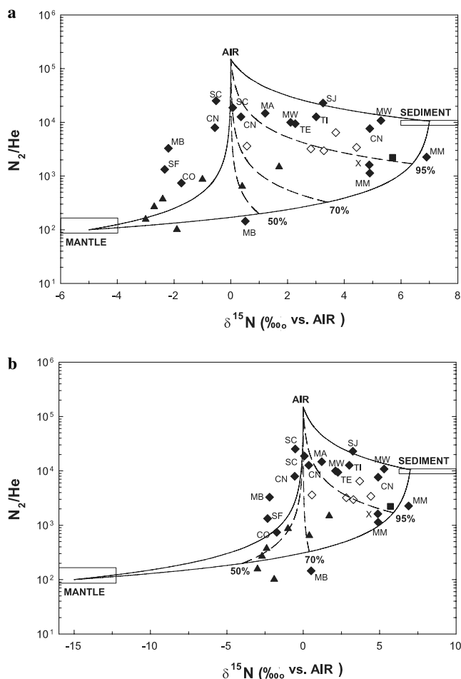
Fig. 6. \delta^{15}\text{N} vs. \text{N}_2/\text{He} diagrams for Nicaraguan geothermal and volcanic gases. Calculations for mixing lines between air, mantle, and sediment are after Sano et al. (2001) and Fischer et al. (2002) and are described in the text. Triangles, Costa Rican gases (Fischer et al., 2002; Zimmer et al., 2004); square, Fuego, Guatemala (Fischer et al., 2002); open diamonds, Nicaragua (Snyder et al., 2003); filled diamonds, Nicaragua (this study). (a) Mixing lines calculated using a mantle \delta^{15}\text{N} = -5\text{‰} . (b) Mixing lines calculated using a mantle \delta^{15}\text{N} = -15\text{‰} . Symbols after Figs. 2 and 4.
