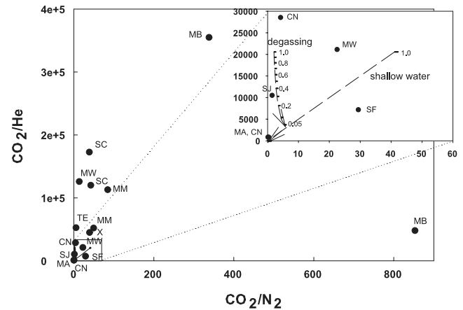
Fig. 5. Diagram of CO 2 3 He vs. CO 2 /N 2 , showing samples from this study and calculated fractionation trends for degassing magma and exsolution from shallow water (calculations explained in Section 5.1.4). Inset shows magnified area of the plot, with calculated trends shown as dashed arrows pointing in the direction of increasing fractionation, and F values as labelled tick marks. Sample CO 2 /N 2 values in this diagram are expressed as CO 2 /N 2, exc . Symbols as in Figs. 2 and 4.
