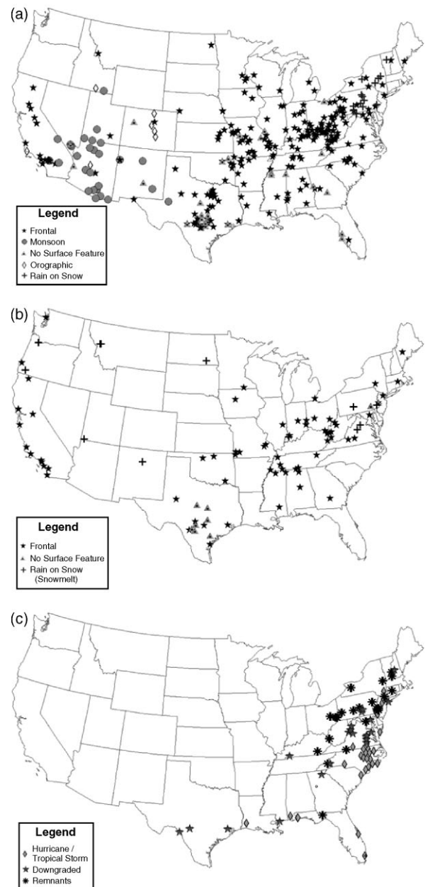
Figure 9. Spatial distribution of deadly storm types by the three dominant flood types, including (a) flash flood, (b) river flood, and (c) tropical system flood. Excludes fatalities from Hurricane Katrina.
