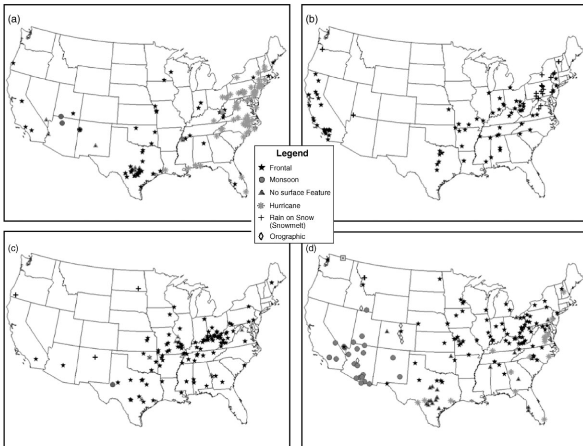
Figure 8. Spatial distribution of deadly storm types (a) fall (Sept–Nov), (b) winter (Dec–Feb), (c) spring (Mar–May), and (d) summer (Jun–Aug).
