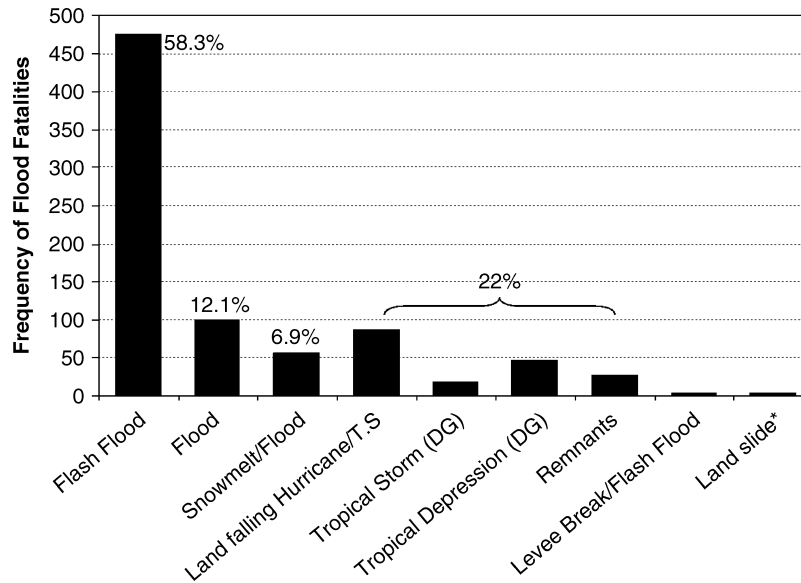
Figure 4. Flood fatalities from 1996 to 2005 separated by flood type. Percentages are given to indicate percent each category contributes to all flood fatalities. DG represents tropical systems downgraded from stronger classification. * Represents high-precipitation events. Excludes fatalities from Hurricane Katrina.
