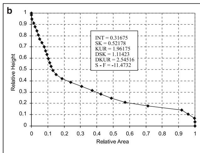
Figure 5. (a) Overlay of a fluvial like watershed basin and Viking image. Drainage channels occur at the high edge of the basin, indicating basin wide extensive erosion, consistent with precipitation runoff origin. (b) Hypsometric curve and attributes of this basin. Characteristics of hypsometric curve clearly shows it is fluvial like. Symbols are the same as those of Figure 4.
