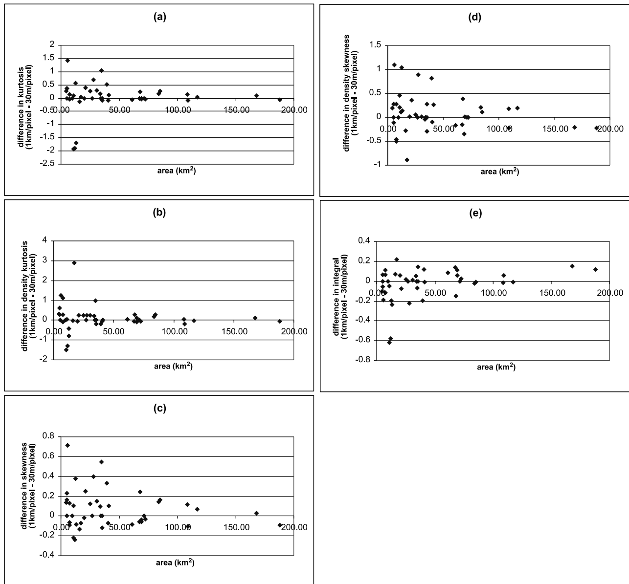
Figure 2. Difference of hypsometric attributes obtained from coarse and fine resolution DEM as a function of basin size. The differences are generally minimized if the basin size is greater than 100 km 2 .
