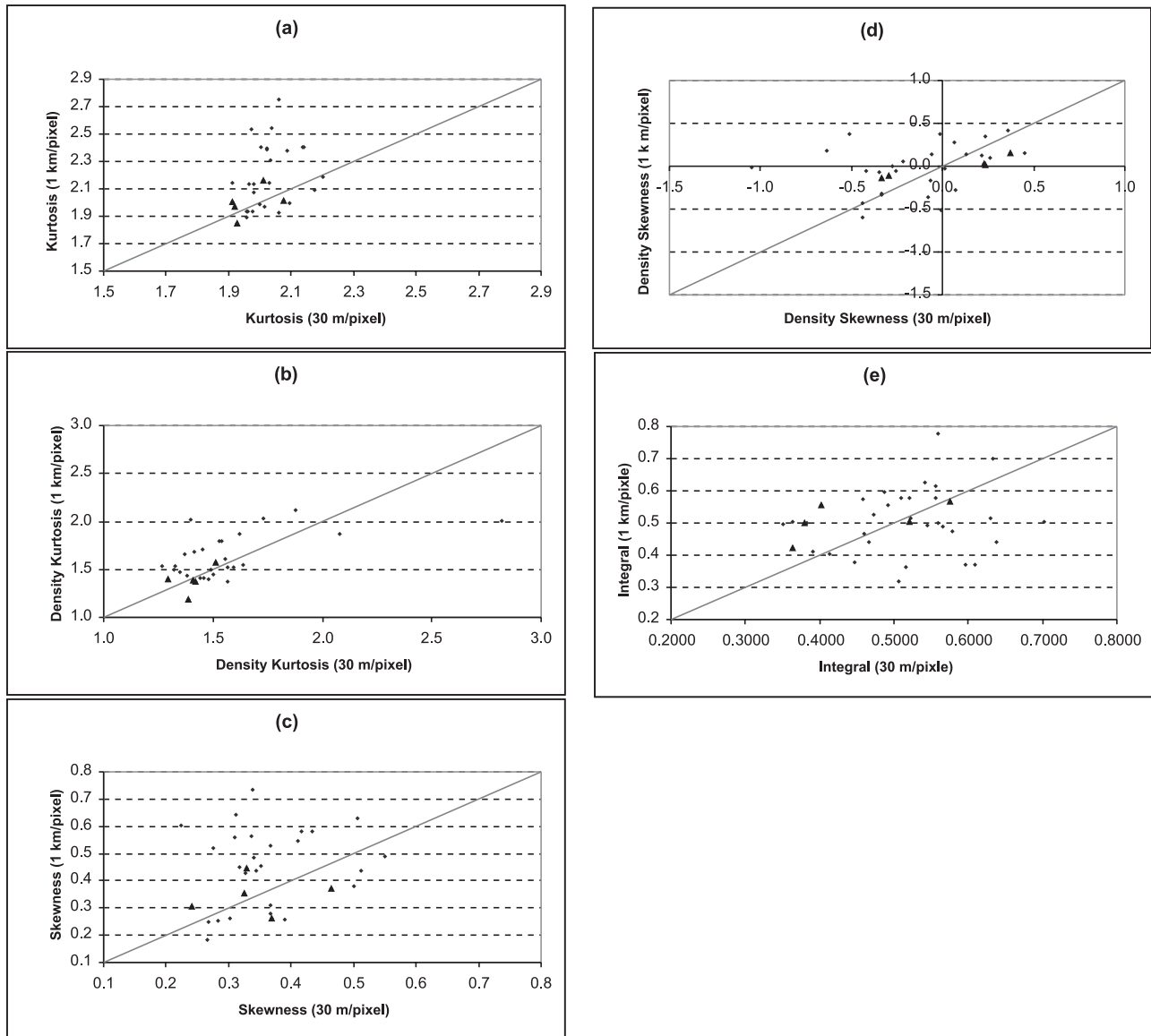
Figure 1. Scatterplots of hypsometric attributes based on 1 km/pixel DEMs vs. those based on 30 m/pixel DEMs. The solid line is the 1:1 line. If the hypsometric attributes are truly resolution independent, the data points should fall on the 1:1 line. Despite the scattering, the general trend of the points follow the 1:1 line. This is especially true for the five basins with area greater than 100 km 2 (shown as triangles).
