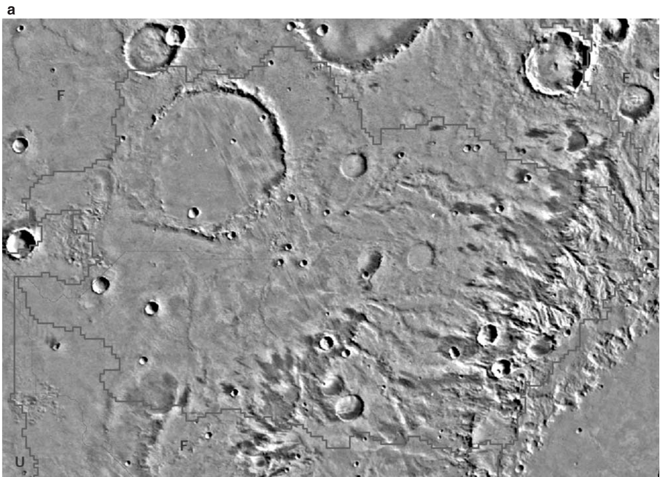
S = Sapping; F = Fluvial; U = Undetermined □ Watershed Boundary - - - Stream Line 0 25 50 100 Kilometers Sinusoidal Projection (central meridian = 20W)
