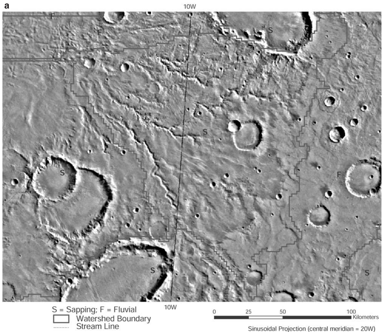
Figure 4. (a) Overlay of a sapping like watershed basin and Viking image. Although there is drainage network, their morphology is consistent with sapping erosion, possibly initiated as fluvial channels. (b) The hypsometric curve and attributes of this basin. Hypsometric curve characteristics clearly look like a sapping basin. INT represents hypsometric integral; SK, skewness of the hypsometric curve; KUR, kurtosis of hypsometric curve; DSK, skewness of hypsometric density function; DKUR, kurtosis of hypsometric density function; F and S discriminant functions for sapping and fluvial basins respectively, see equations (1) and (2).
