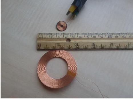
Figure 2. Receiver Coils
