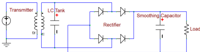
Figure 3. Wireless Charging Circuit
