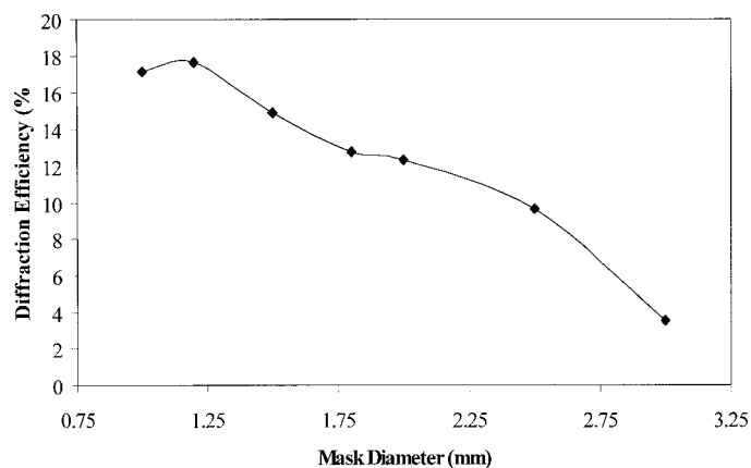
FIG. 3. 324.7 nm Cu first-order diffraction efficiency as a function of aperture size.
